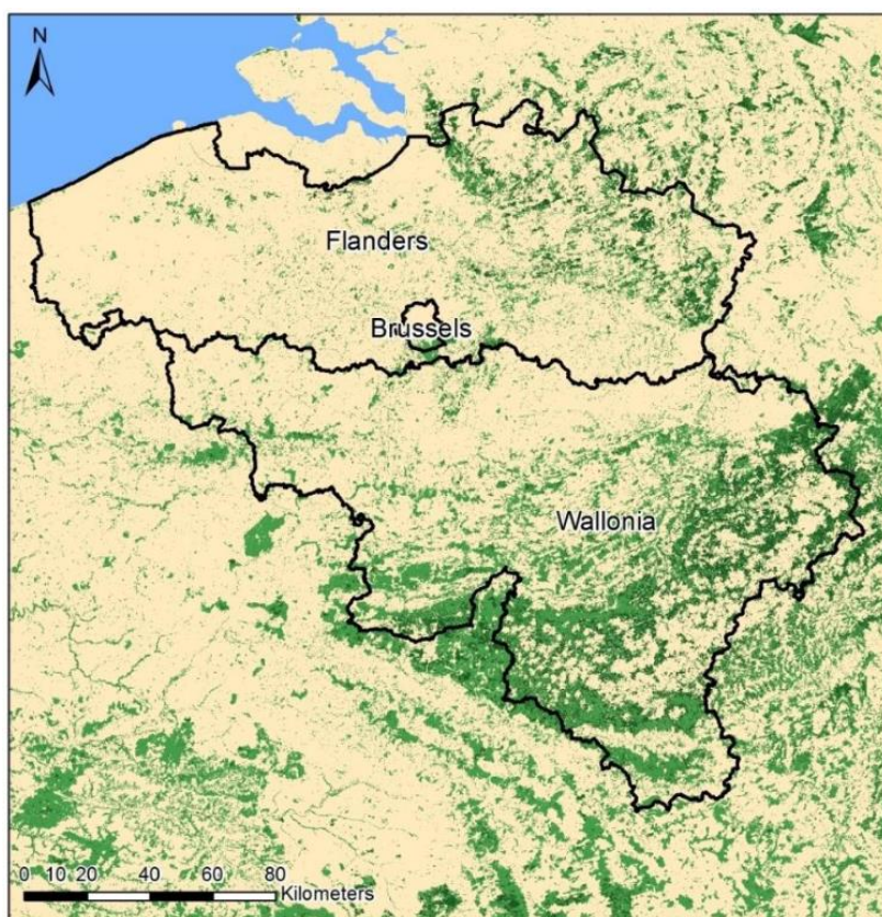
Figure 3-48. Forest cover in the three regions of Belgium in green (ULiège, 2018).
