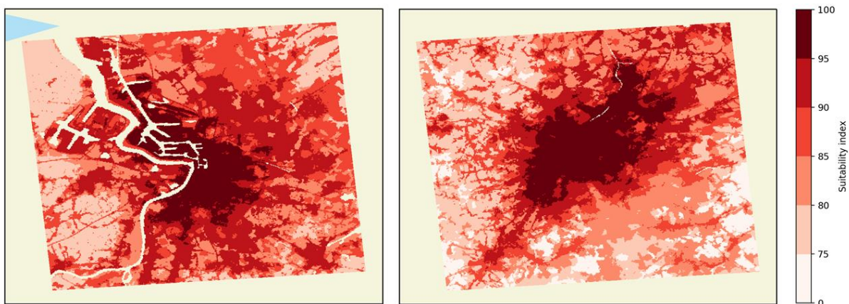
Figure 3-15. Suitability for the survival of Aedes albopictus (Tiger mosquito), as the average over the period 2008-2017, for Antwerp (left) and Brussels (right). Source: Copernicus Climate Change Service & VITO, 'Climatic suitability of the Aedes albopictus mosquito in European cities from 2008 to 2017 2 .
