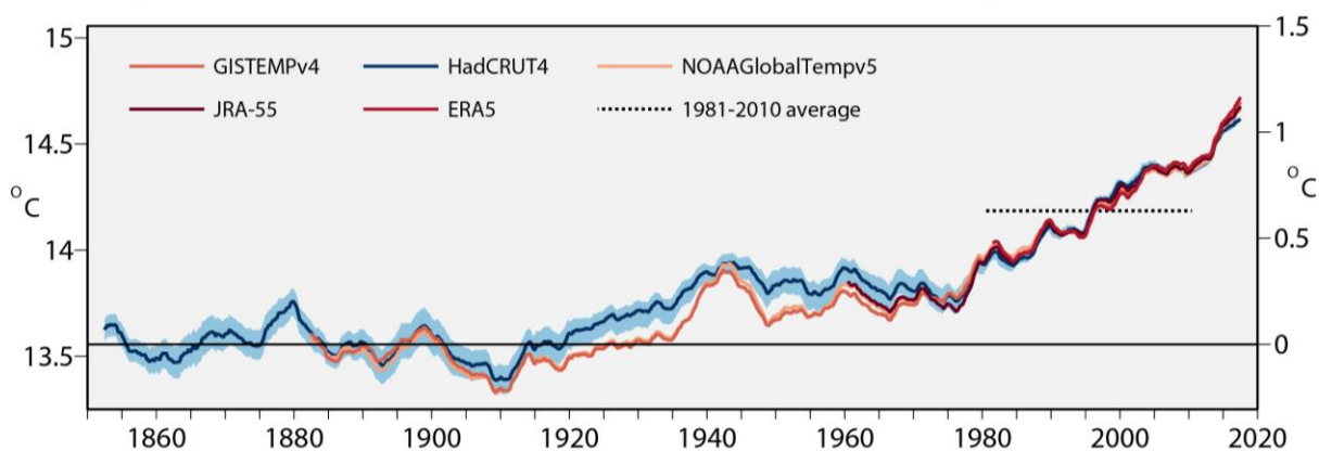
Figure 1-1. Annual average, global 60-month average near-surface air temperature relative to the pre-industrial period. Source: Copernicus Climate Change Service.
