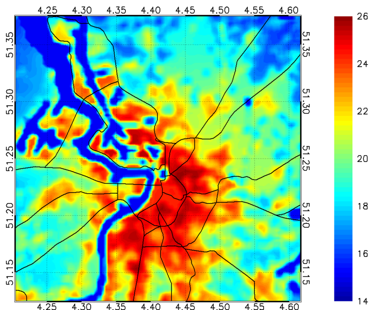
Figure 2-11. Mean annual number of heatwave days simulated for the Antwerp area for the period 2081-2100 under scenario RCP8.5. Source: Hooyberghs et al. (2015).
